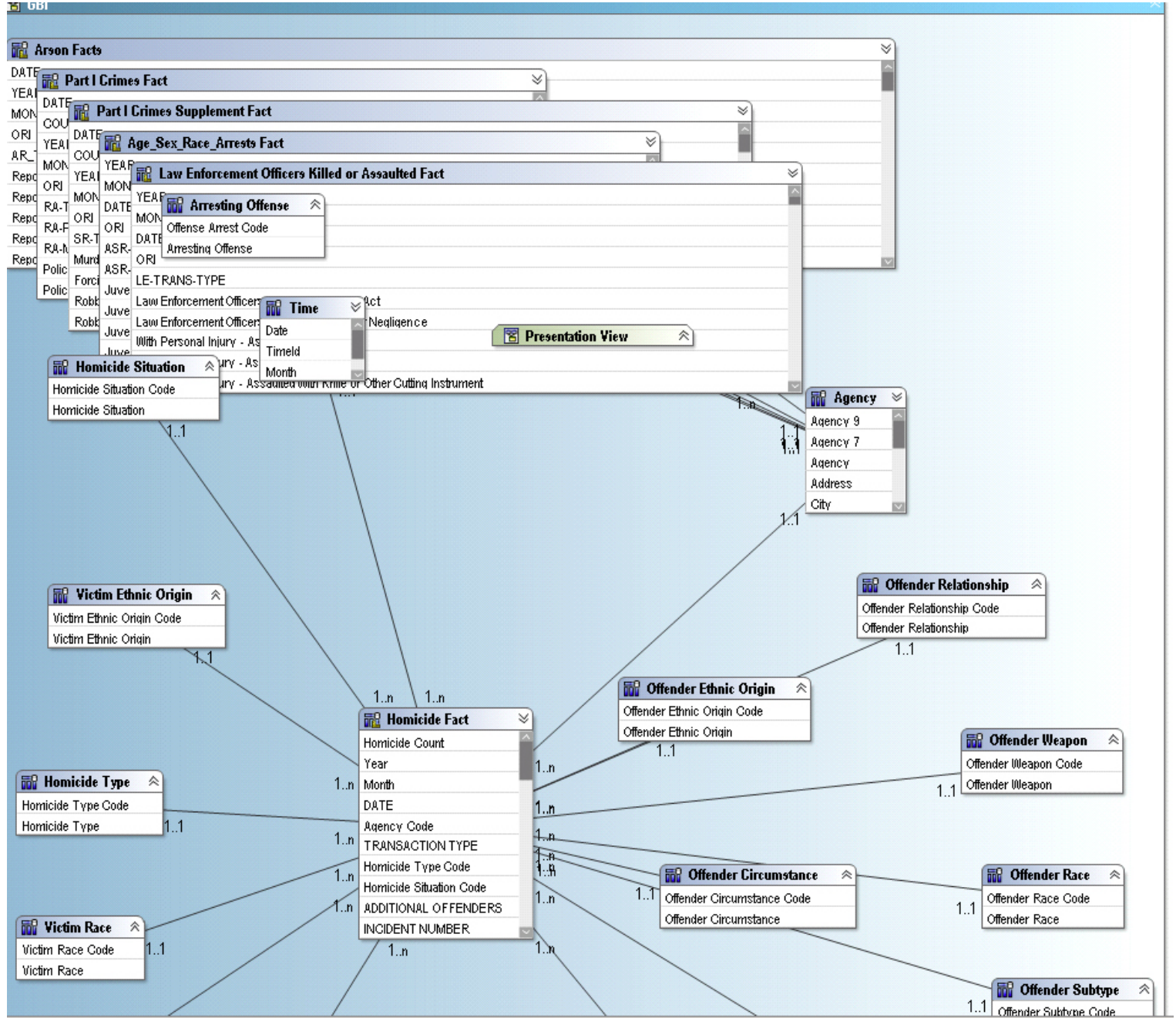
COGNOS Frame Work Manager Star Schema Diagram
